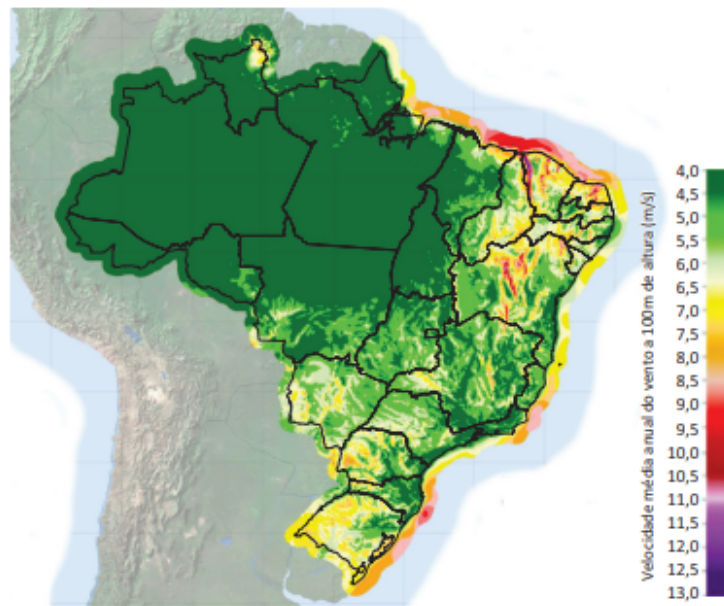
Figure 1 | Brazilian Wind Power Average annual wind speed at 100 meters high (m/s).
