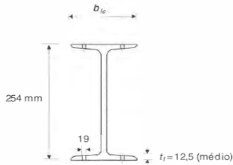
Figure 2. Proposed beam (M. and W. Pfeil (2009)).
