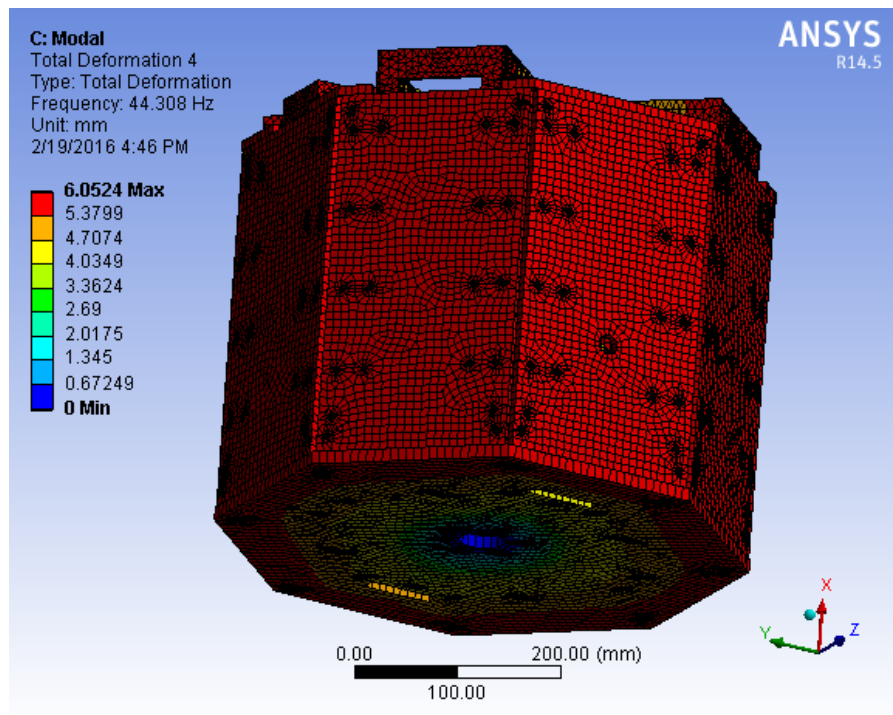
Figure 13: longitudinal mode of vibration using the aluminium alloy and carbon fiber composite material
