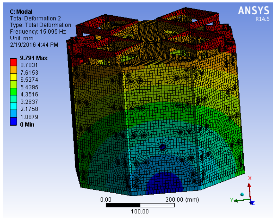
Figure 11: First lateral mode of vibration using the aluminium alloy and carbon fiber composite material
